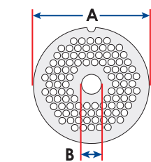
A. 3-1/4" Plate Diameter B. 0.450" Center Bore
