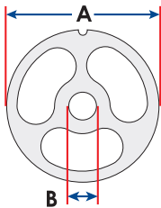
A. 3-1/4" Plate Diameter B. 0.450" Center Bore
